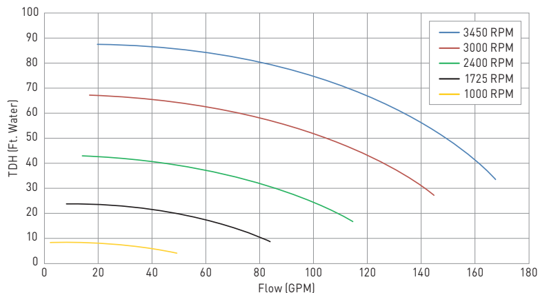
TRISTAR VS 950 PERFORMANCE COMPARISON
