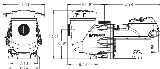
TRISTAR VS 950 DIMENSIONS (INCHES)
